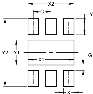
U-DFN1616-6 (Type G)
