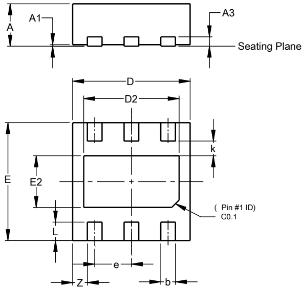
U-DFN1616-6 (Type G)
