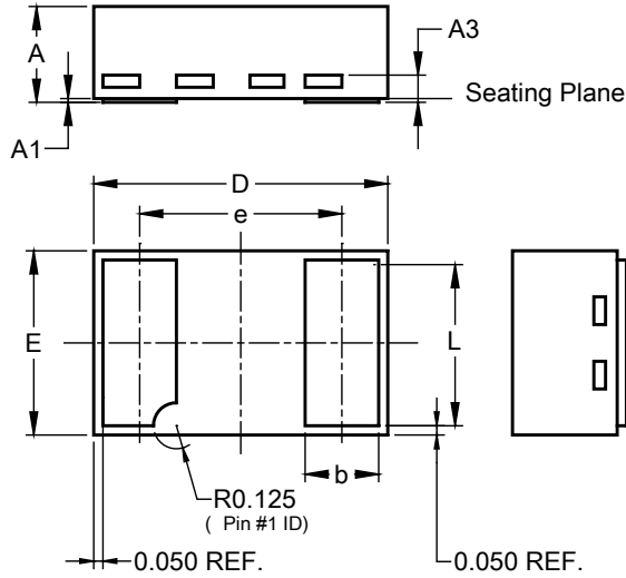
U-DFN1610-2 (Type C)
