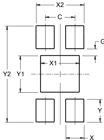
U-DFN1218-4
