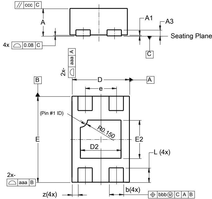
U-DFN1218-4
