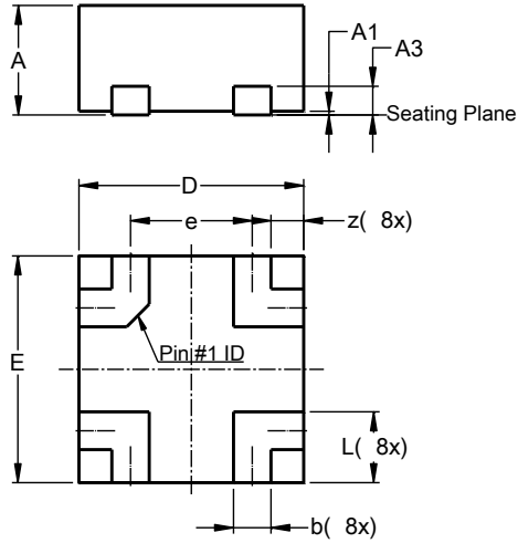
U-DFN1212-4
