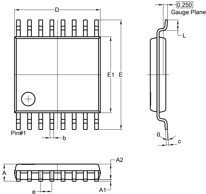
TSSOP-16 (Type CJ)
