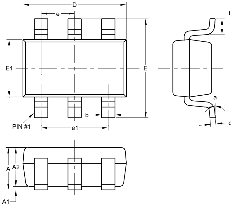
TSOT26 (Type SM)
