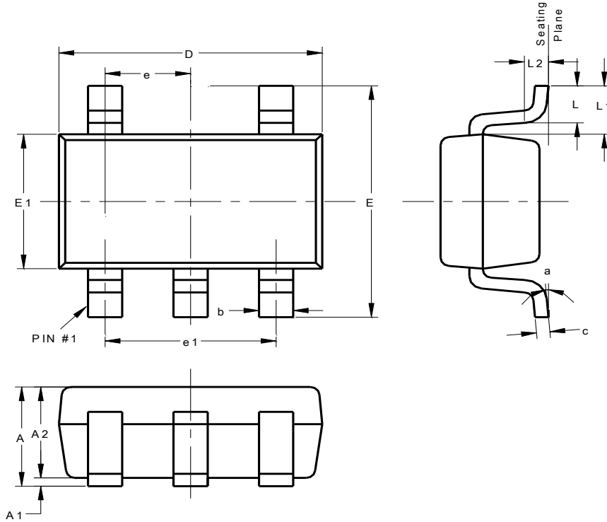
TSOT25 (Type SM)
