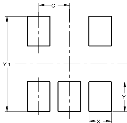
TSOT25 (Type SM)
