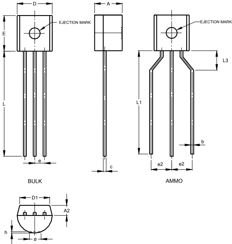
TO-92 (Type B)
