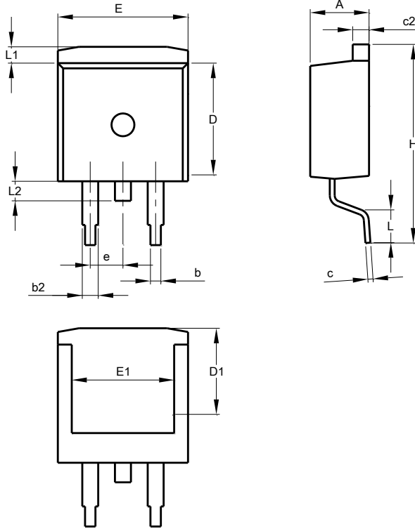
TO263AB (D2PAK) (Type BR)
