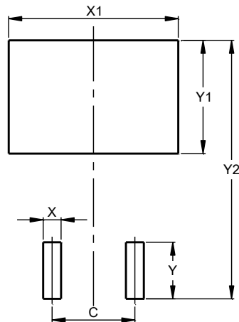
TO263AB (D2PAK) (Type BR)
