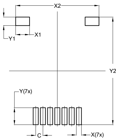
TO263-7 (Type WH)
