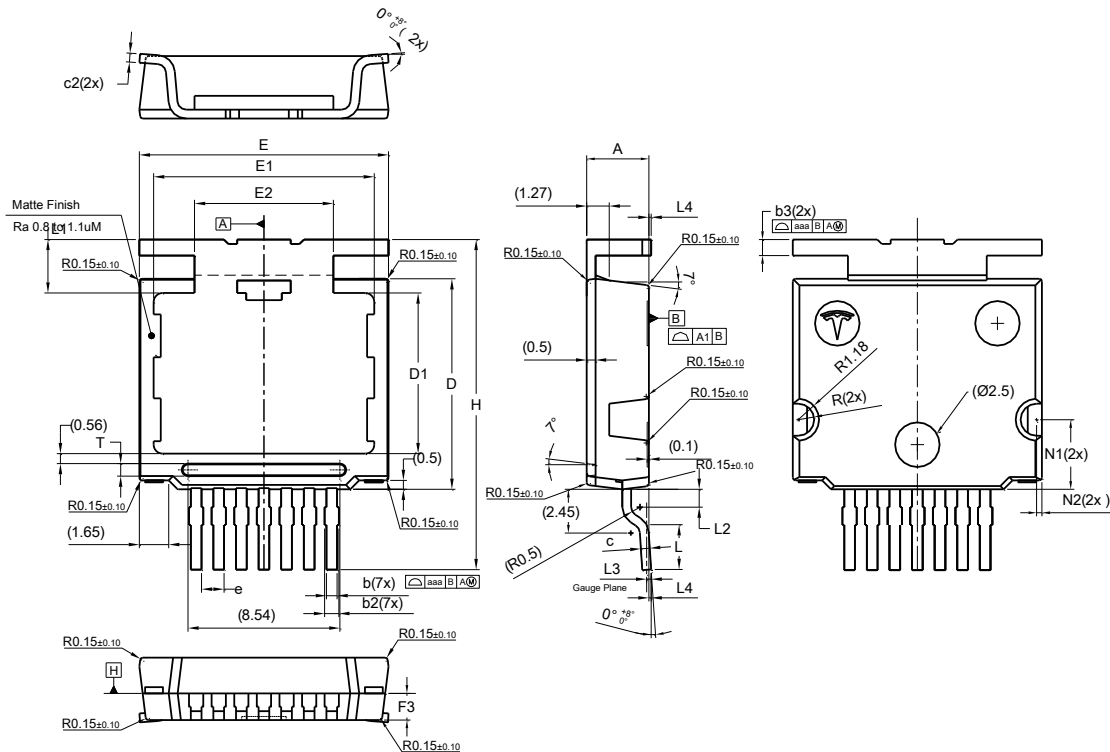
TO263-7 (Type WH)
