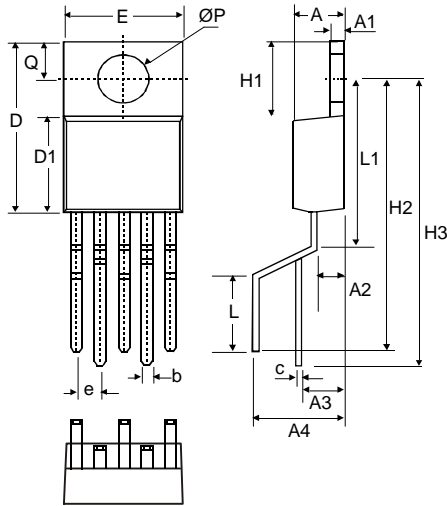
TO220-5(R)
