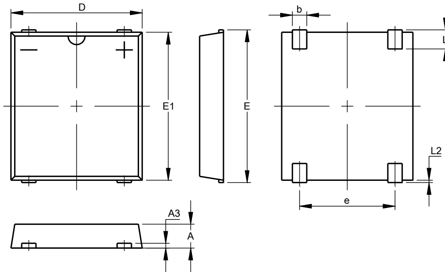
T-DFN5564-4
