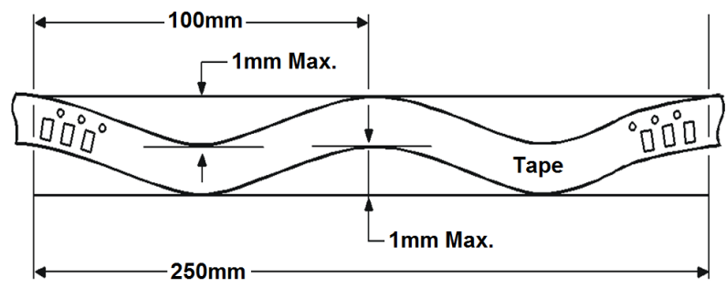
Camber (Top View) Allowable camber to be 1mm/100mm tape, non-cumulative
