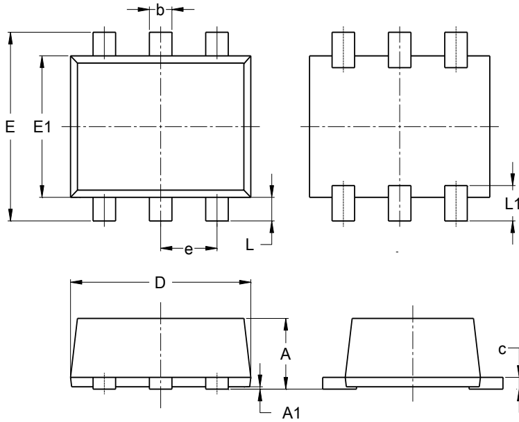
SOT563 (Type TH)
