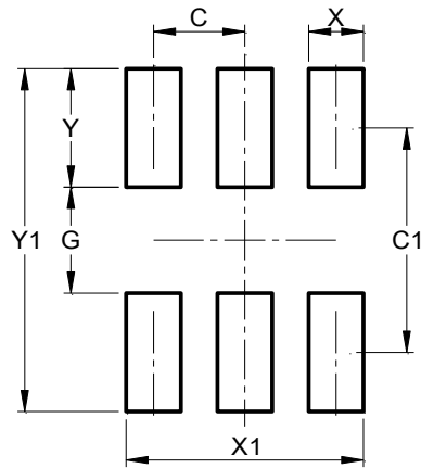
SOT563 (Type TH)
