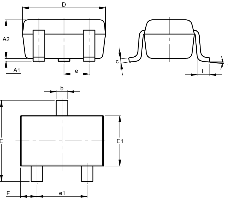
SOT323 (Standard)
