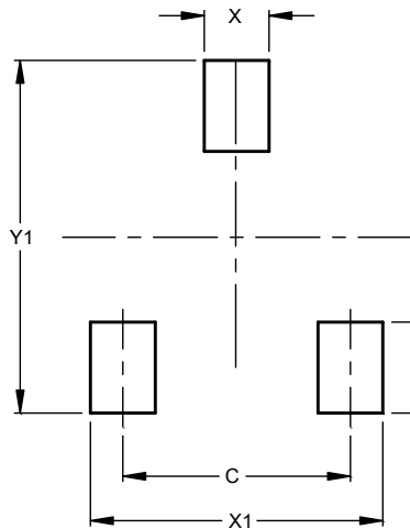
SOT23 (Type BR)
