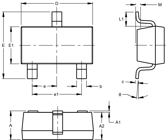
SOT23 (Type BR)
