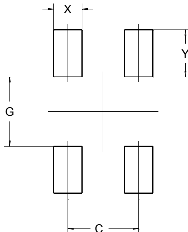
SOT23-4 (Type C)
