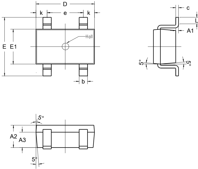
SOT23-4 (Type C)
