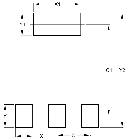
SOT223 (Type DN)
