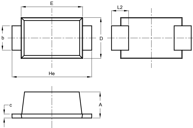
SOD123F (Type 9)
