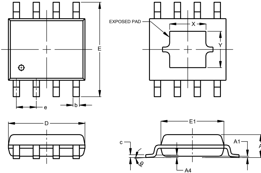
SO-8EP (Type B)
