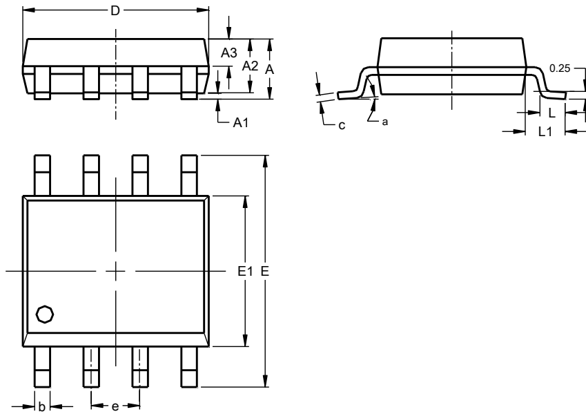
SO-8 (Type TH)
