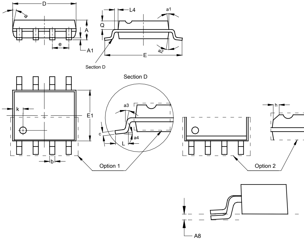
SO-8 (Type CJ)
