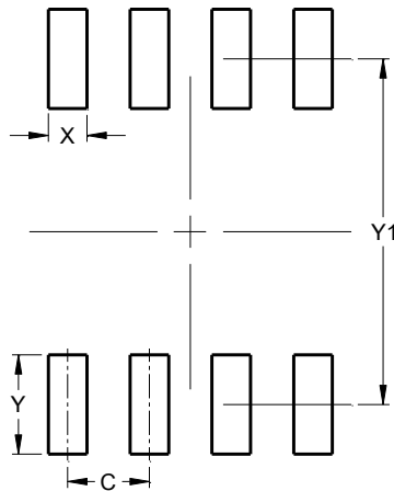
SO-8 (Type A1)
