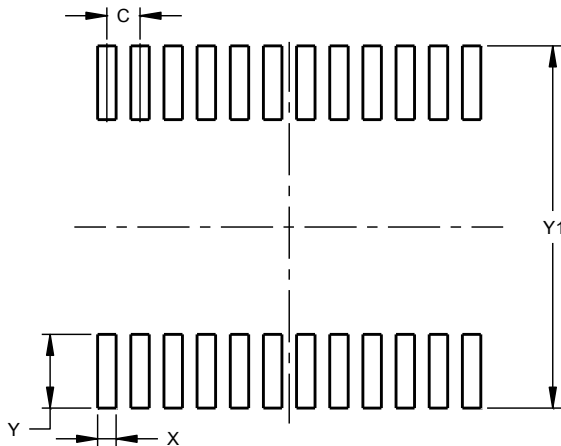
SO-24 (Type TH)
