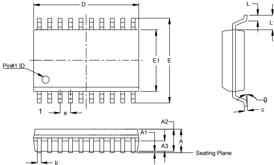
SO-20 (Type TH)
