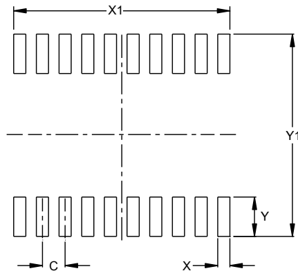
SO-20 (Type TH)
