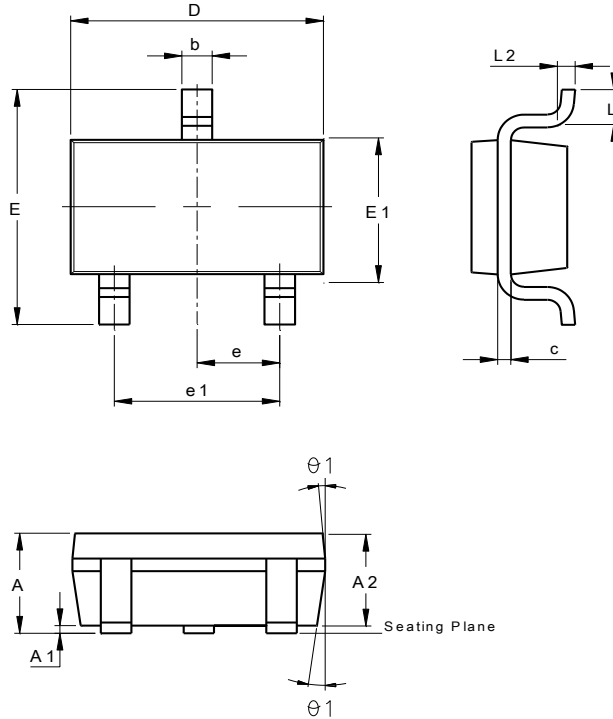
SC59 (Type A1)
