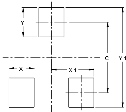
SC59 (Type A1)
