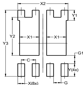
PowerDI5060-8 SWP (Type D Standard)
