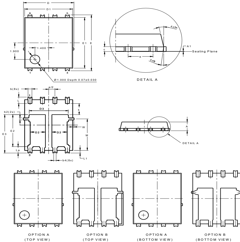
PowerDI5060-8 SWP (Type D Standard)
