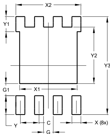
PowerDI5060-8 (Type K)
