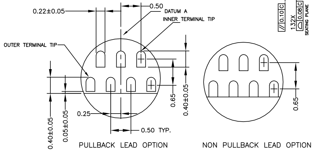
DETAIL A (SCALE 3:1)
