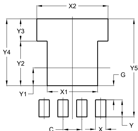
PD56LF-4
