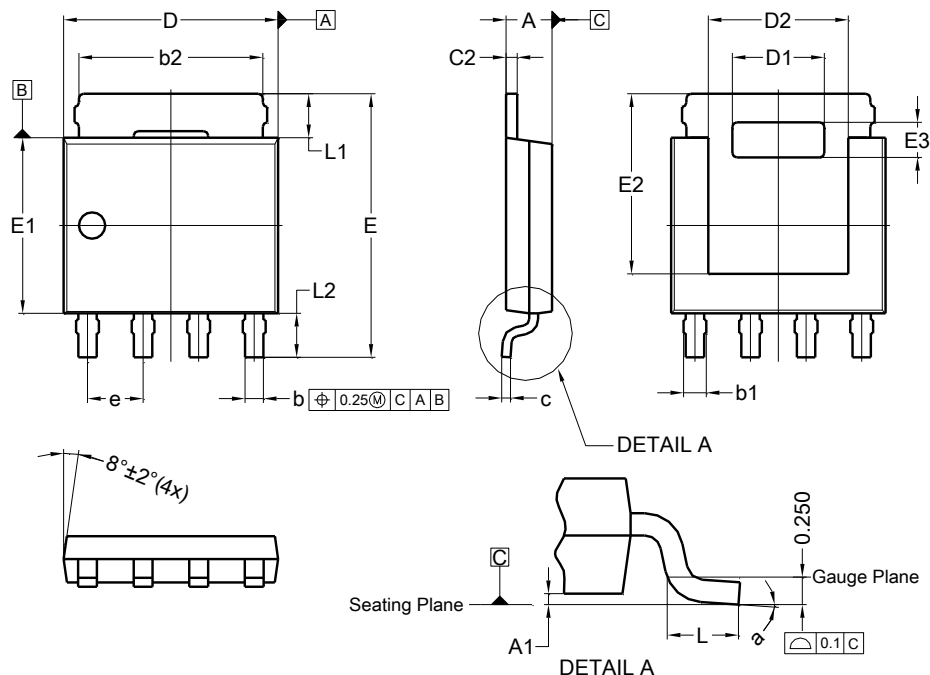
PD56LF-4
