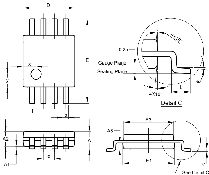
MSOP-8
