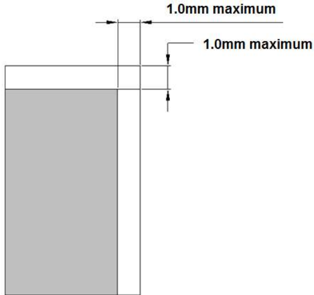
Maximum Component Rotation Top View
