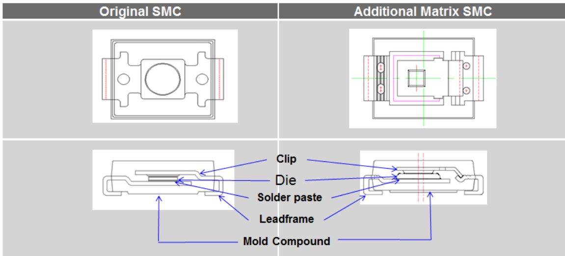
Figure 4: Comparison of SMC Package Construction for SKY, GPP and Unidirectional TVS products
