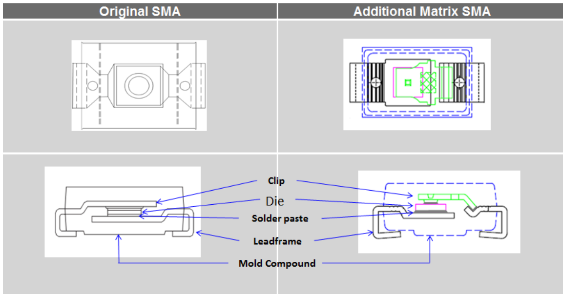
Figure 1: Comparison of SMA Package Construction for SKY and SBR products
