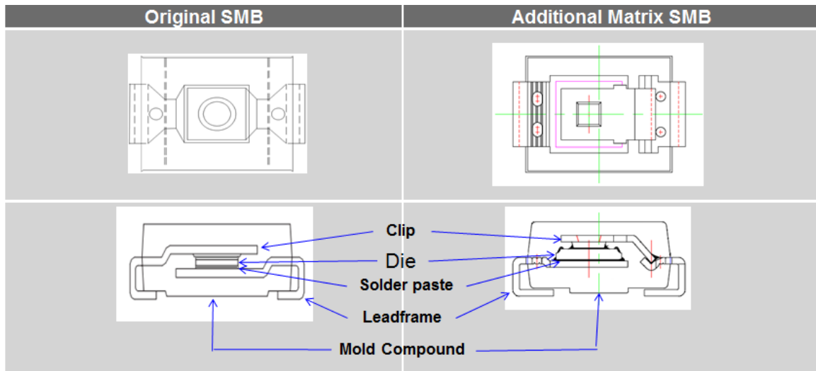
Figure 2: Comparison of SMB Package Construction for SKY, GPP, Zener and Unidirectional TVS products
