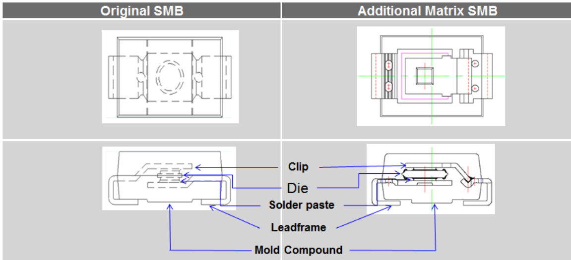
Figure 3: Comparison of SMB Package Construction for Bidirectional TVS products
