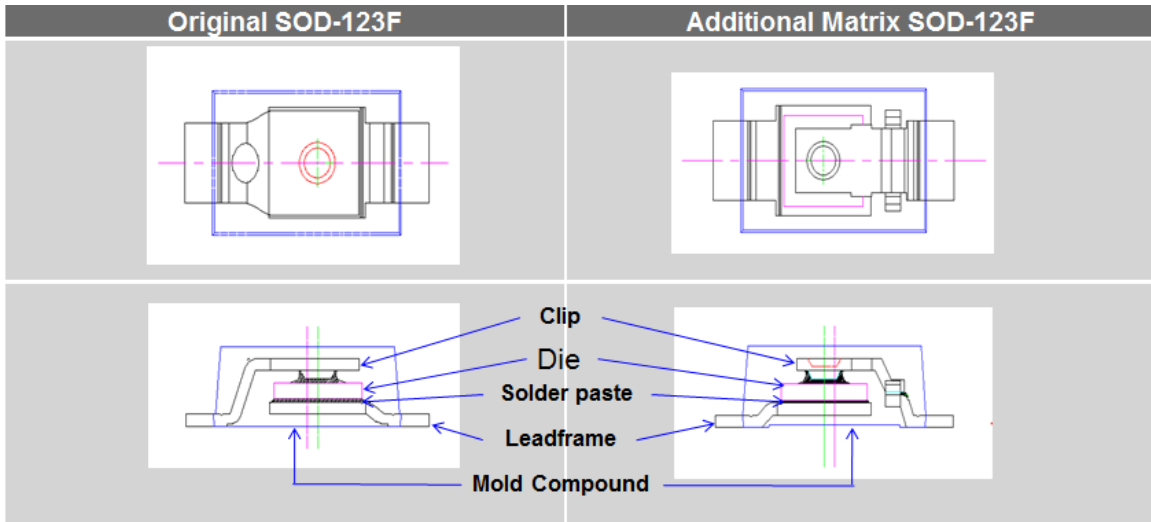
Figure 6: Comparison of SOD-123F Package Construction for SKY, SBR and GPP products
