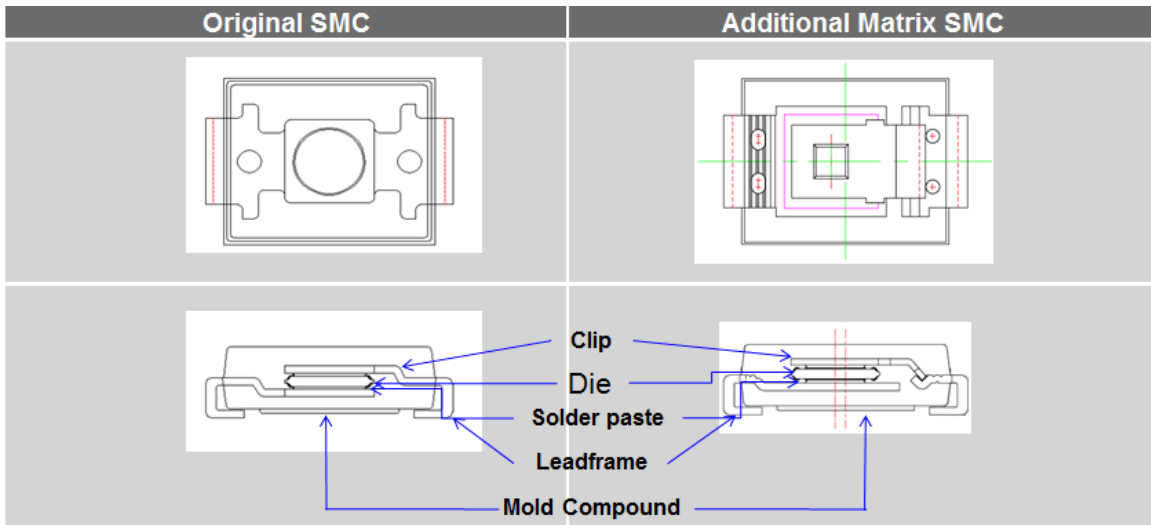
Figure 5: Comparison of SMC Package Construction for Bidirectional TVS products
