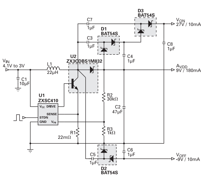
ZXSC410 as Triple Output TFT Bias
