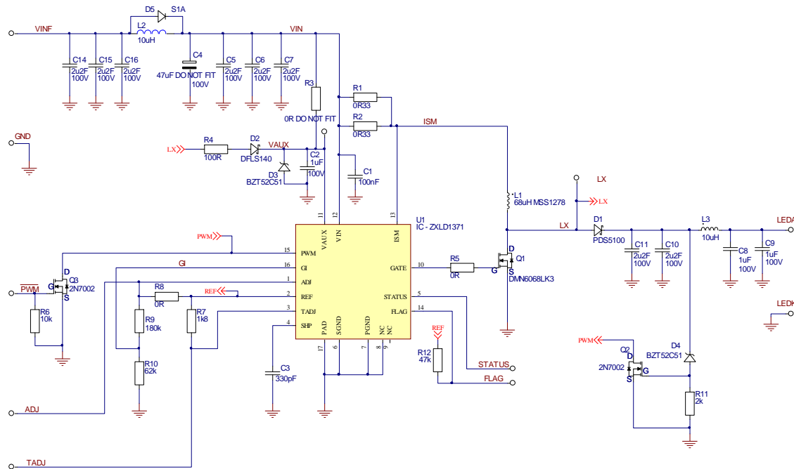
Figure 2: ZXLD1371EV3 evaluation board Schematic
