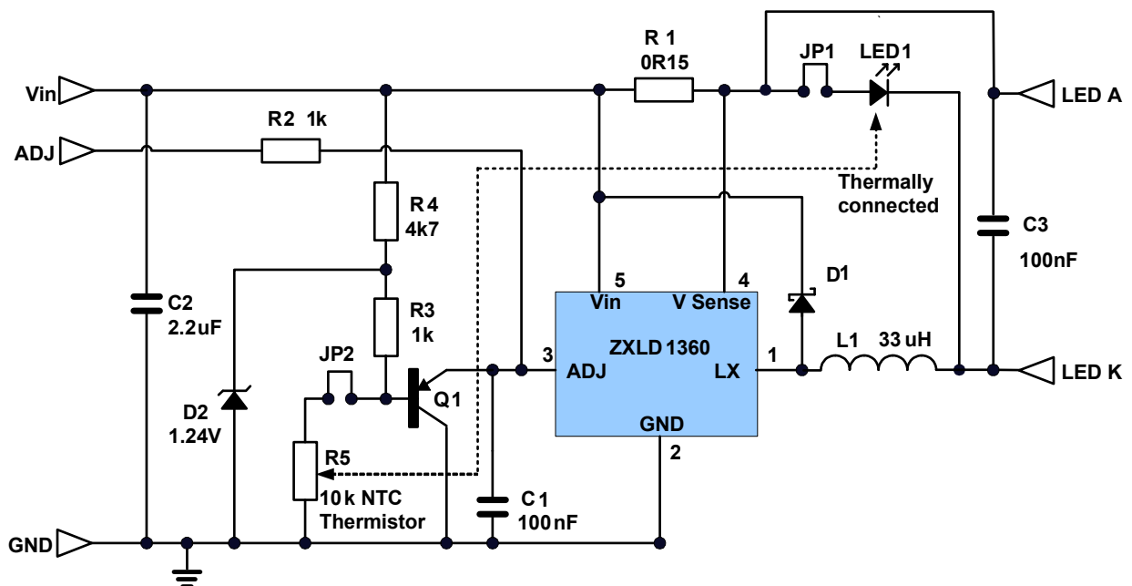
Figure 2: Schematic for the evaluation board ZXLD1360EV8
