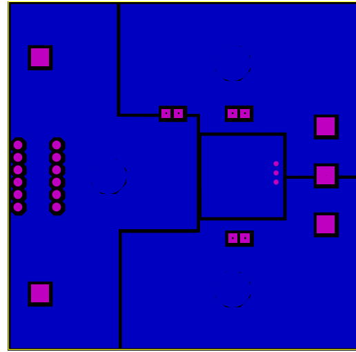
Figure 5: Bottom View
