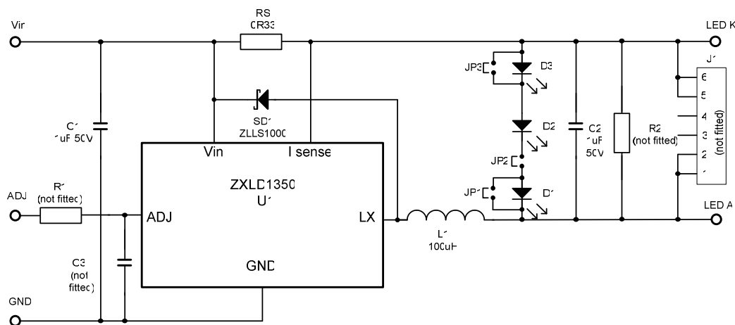
Figure 2: Schematic for the evaluation board ZXLD1350EV7
