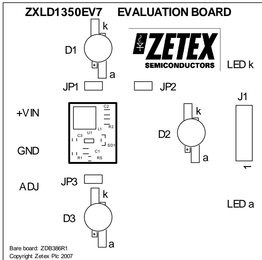
Figure 3: Component layout
