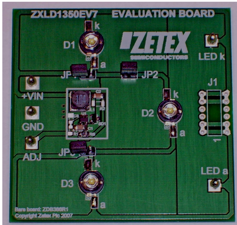
Figure 1: ZXLD1350EV7 evaluation board
