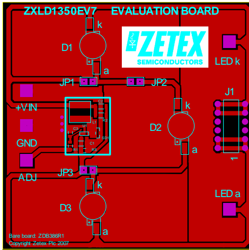
Figure 4: Top View
