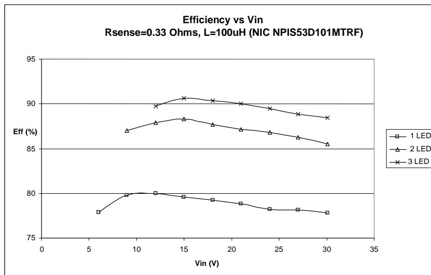
Figure 6: Efficiency vs supply voltage
