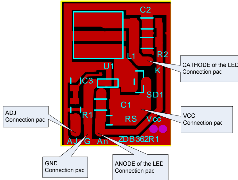
Figure 3: Component layout
