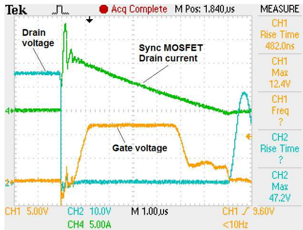
Figure 4: Operating waveforms in QR mode with a 10mΩ 100V synchronous MOSFET
