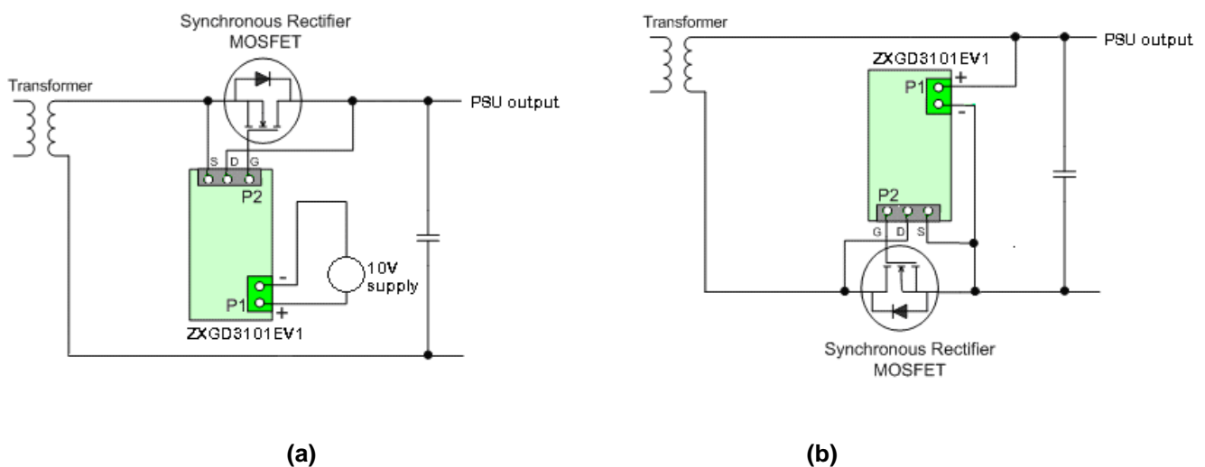
Figure 3: Test options for ZXGD3101EV1 a) high side and b) low side
