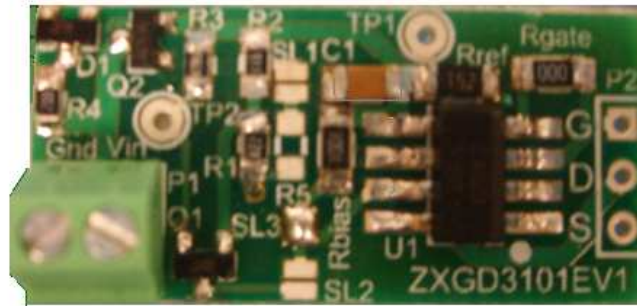
Figure 1 Evaluation board layout and connection diagram
