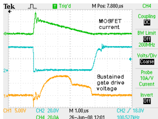
Figure 7 DCM gate drive voltage a) showing premature turn off and b) premature turn-off and oscillations eliminated using a constant bias current source
