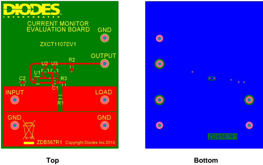
Fig. 2 – ZXCT1107EV1 PCB Layout
