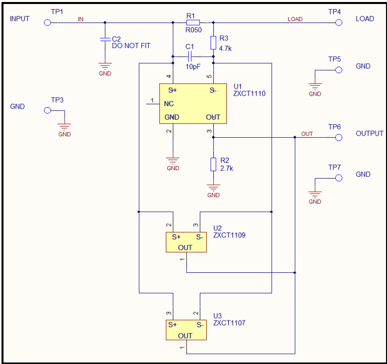
Fig. 1 – ZXCT1107EV1 Schematic
