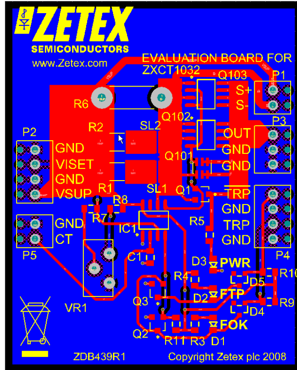
Figure 1 Evaluation board components' layout
