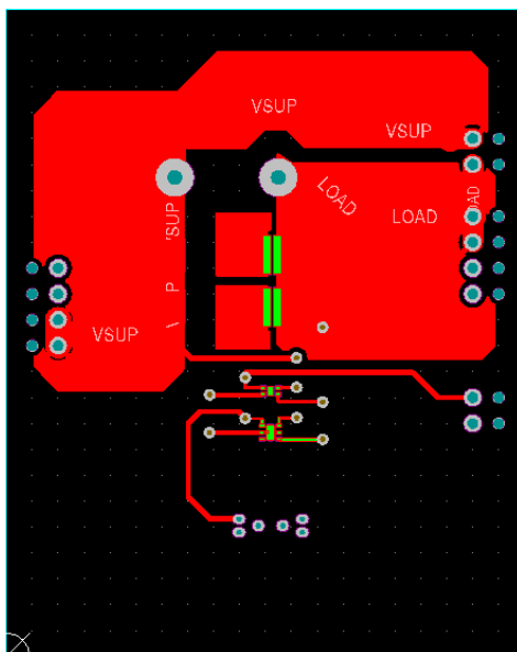
Top Copper
