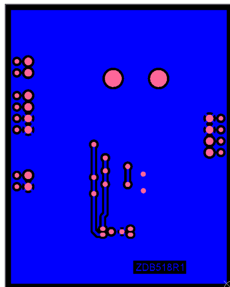
Bottom Copper
