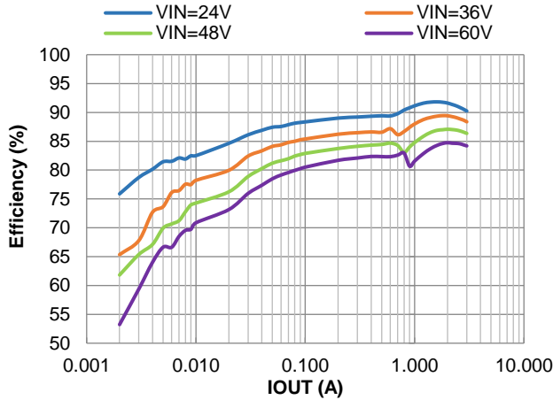
Figure 7. PFM Efficiency vs. IOU T , V OUT =5V, L=6.5µH
