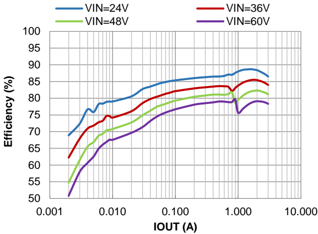
Figure 9. PFM Efficiency vs. IOU T , V OUT =3.3V, L=5.5µH
