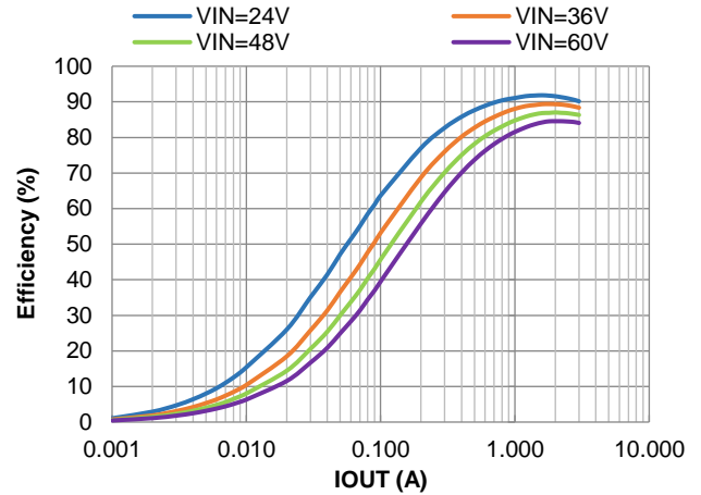
Figure 8. PWM Efficiency vs. IOU T , V OUT =5V, L=6.5µH
