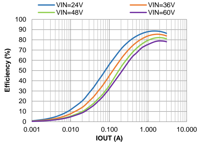
Figure 10. PWM Efficiency vs. IOU T , V OUT =3.3V, L=5.5µH
