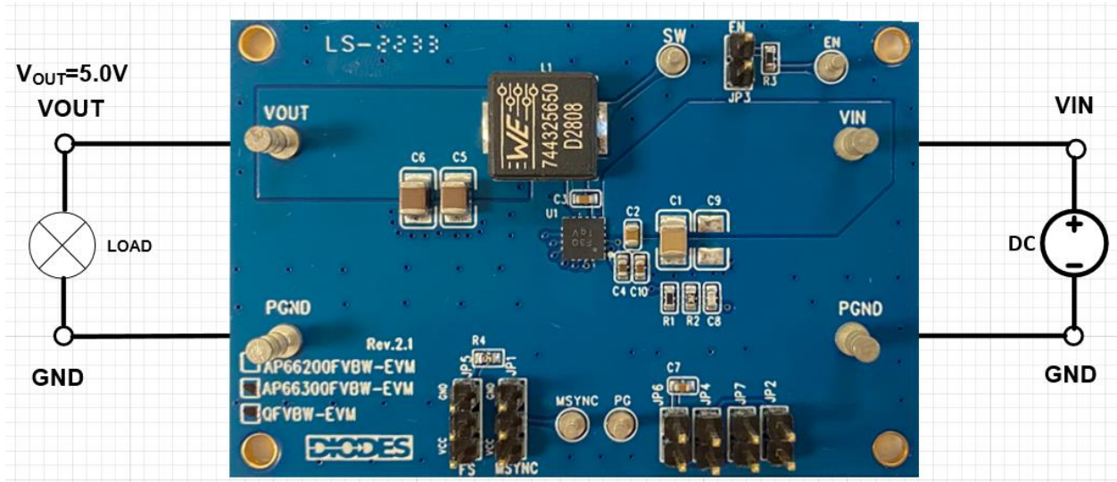
Figure 1. AP66300QFVBW-EVM
