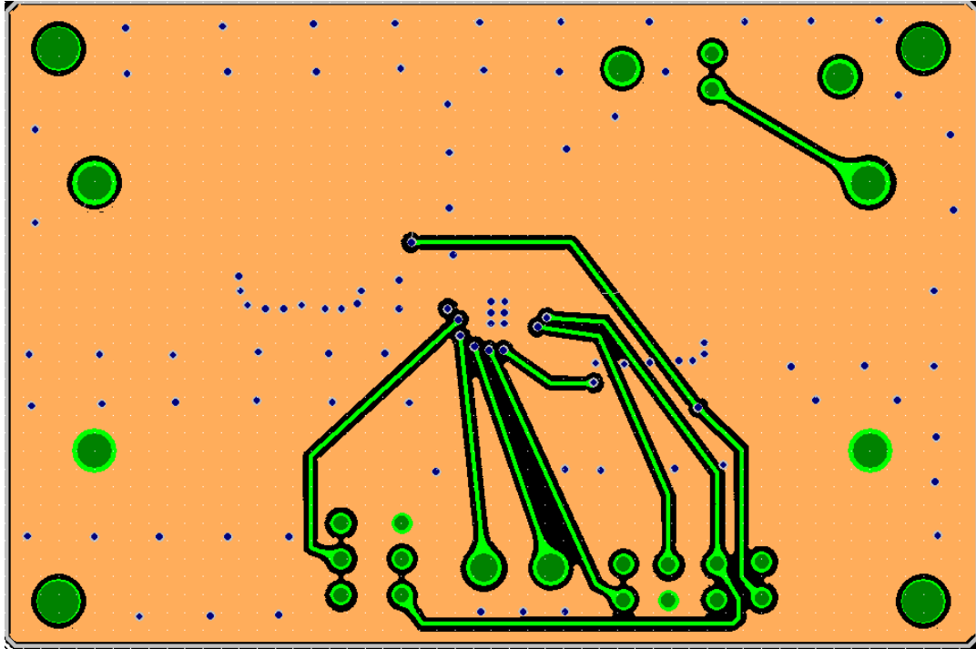
Figure 5. AP66300QFVBW-EVM – Layer 3
