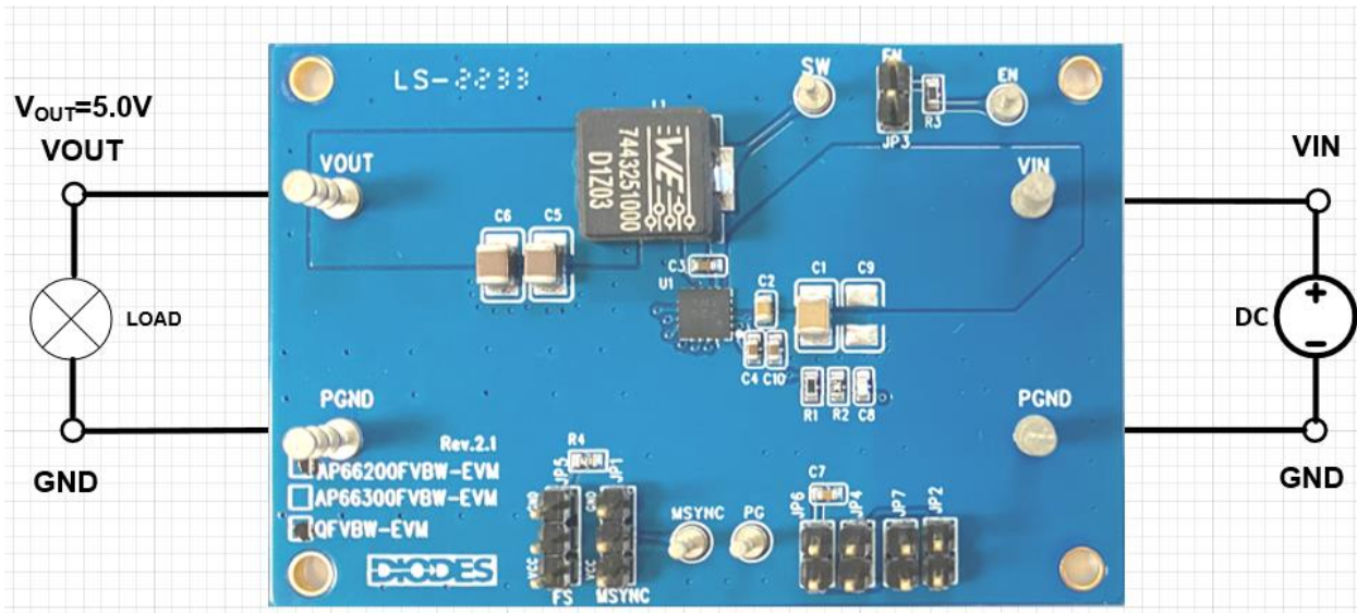
Figure 1. AP66200QFVBW-EVM
