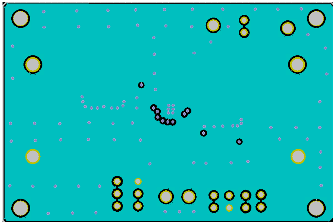
Figure 4. AP66200QFVBW-EVM – Layer 2
