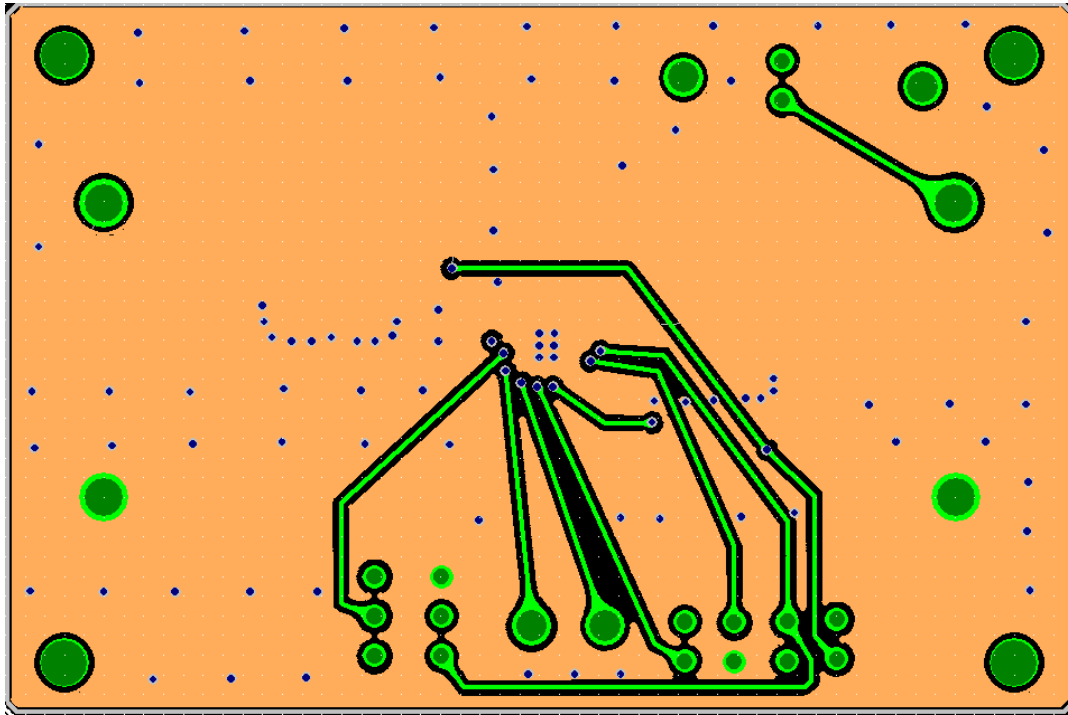
Figure 5. AP66200QFVBW-EVM – Layer 3
