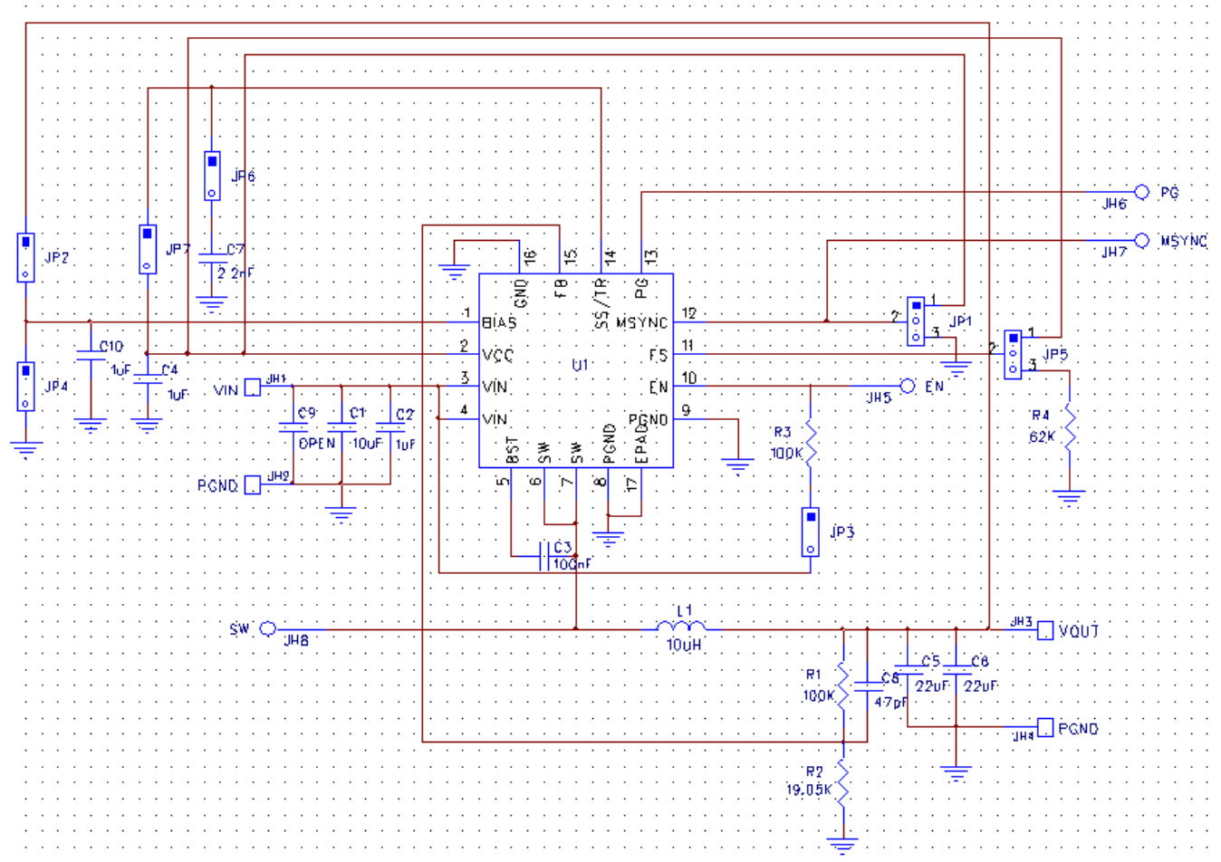
Figure 2. AP66200QFVBW-EVM Schematic
