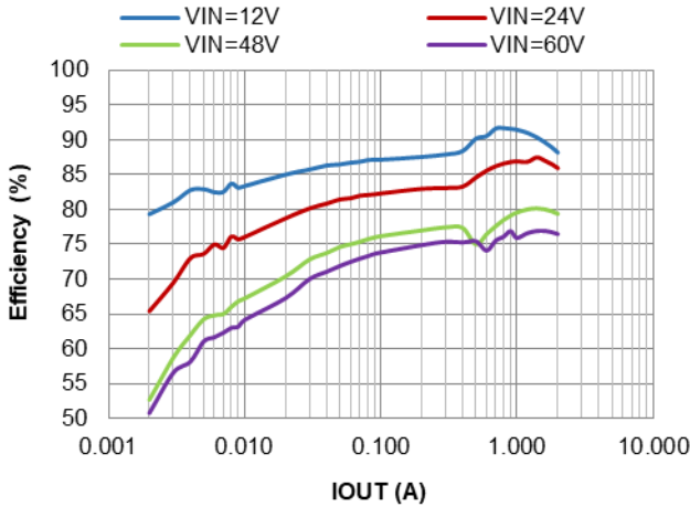
Figure 9. PFM Efficiency vs. IOU, V_{out}=3.3V , L=8.2\mu H
