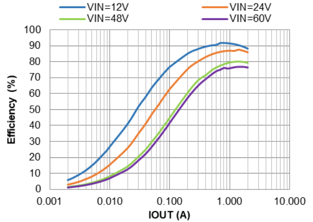
Figure 10. PWM Efficiency vs. IOU, V_{out}=3.3V , L=8.2\mu H
