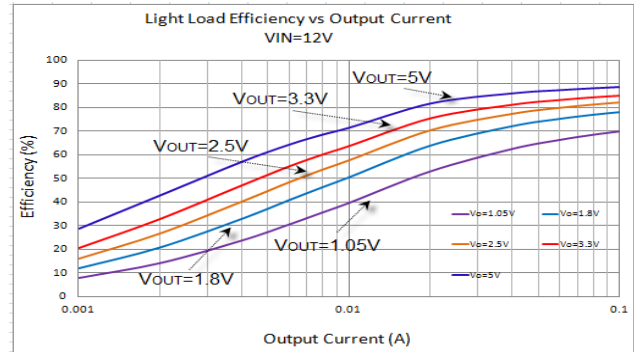
Figure 4. Light Load Efficiency
