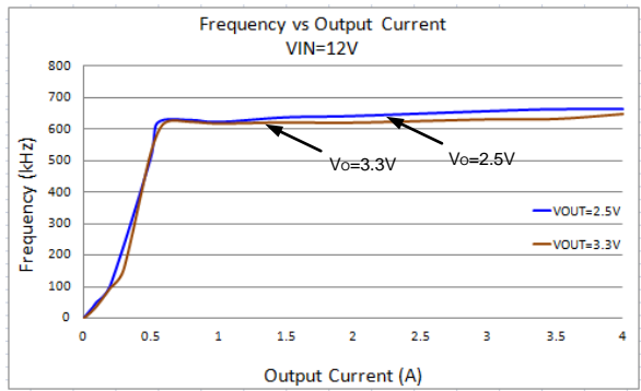
Figure 4. Frequency vs Output Current
