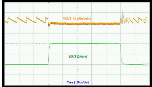
Figure 2. Load Transient 0 to 4A
