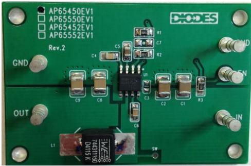
Figure 1. Evaluation Board (Rev2)
