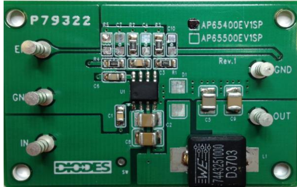
Figure 1. Evaluation Board
