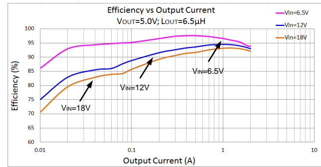
Figure 4. Efficiency (VOUT=5.0V)
